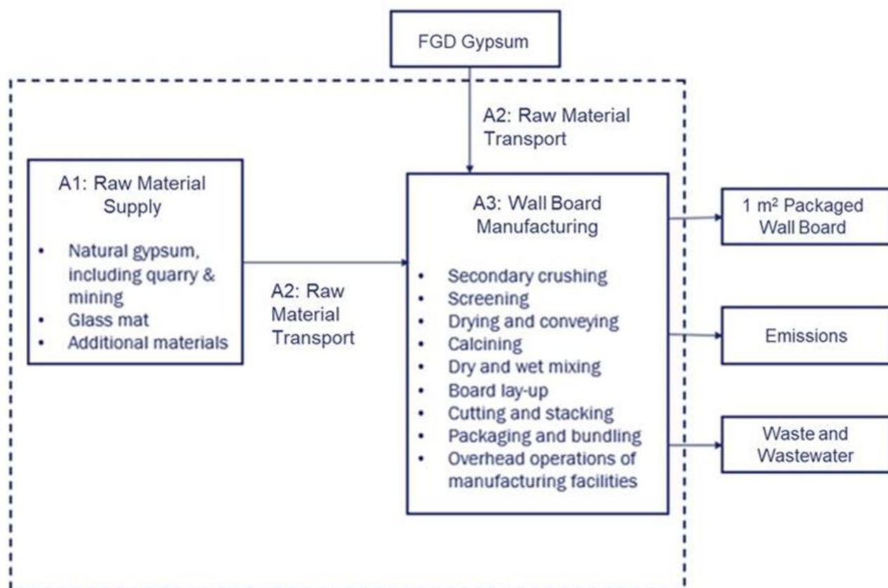
Figure 3-1: Simple flow chart providing details on the Product Stage (A1 to A3) for 1/2" DensShield® Tile Backer
