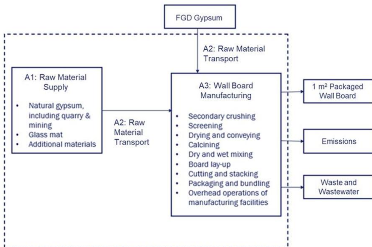
Figure 3-1: Simple flow chart providing details on the Product Stage (A1 to A3) for 5/8" DensGlass® Fireguard® Sheathing
