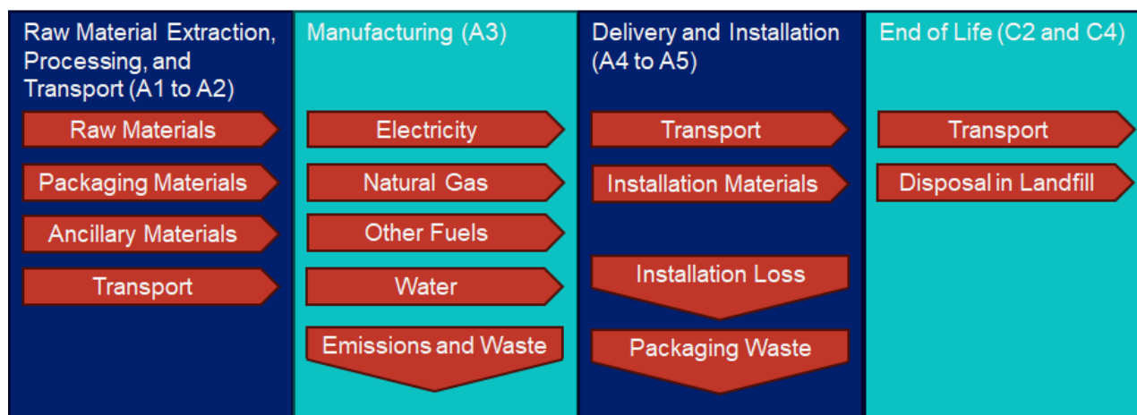
Figure 1-1: Simplified process flow diagram for 5/8" DensGlass® Fireguard® Sheathing
